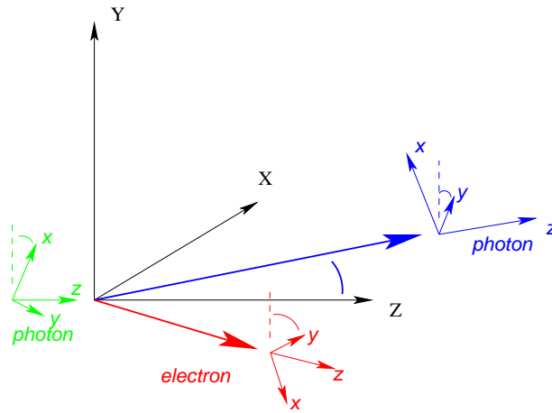
Figure 17.1: The interaction frame and the particle frames for the example of Compton scattering. The momenta of all participating particle lie in the x - z -plane, the scattering plane. The incoming photon gives the z direction. The outgoing photon is defined as particle 1 and gives the x -direction, perpendicular to the z -axis. The y -axis is then perpendicular to the scattering plane and completes the definition of a right handed coordinate system called interaction frame . The particle frame is defined by the Geant4 routine G4ThreeMomentum::rotateUz() .
